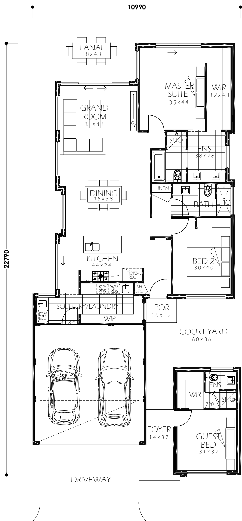
FLOOR PLAN SCALE 1 : 100
