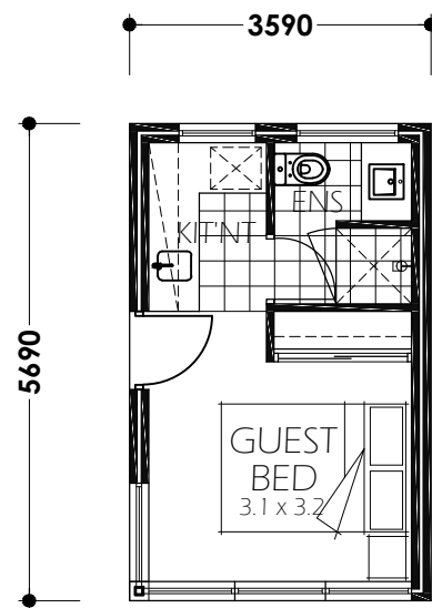
ALTERNATIVE DESIGN SCALE 1 : 100
